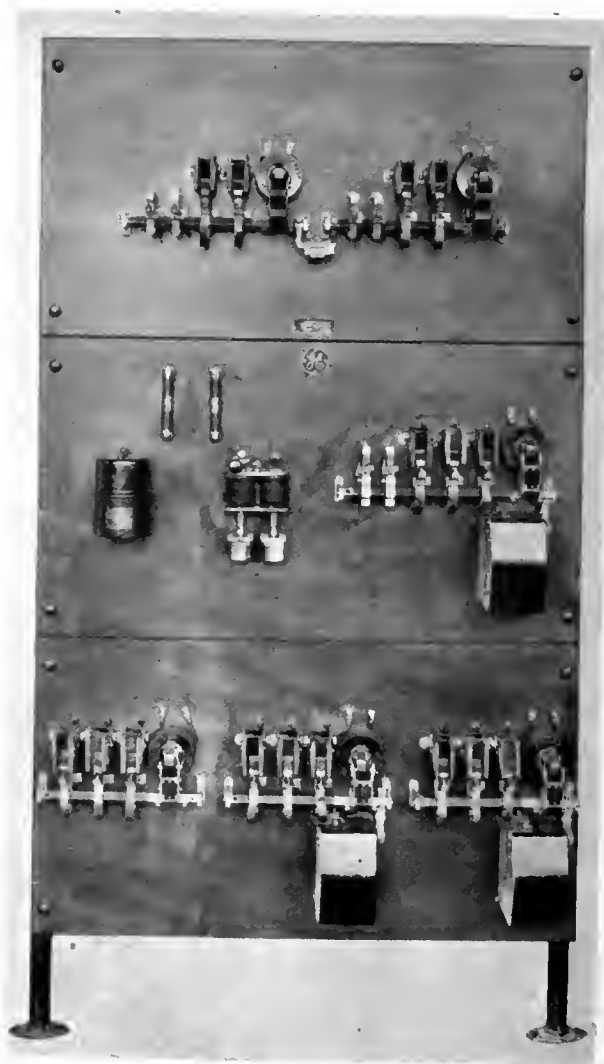
FIG. 1. TYPICAL 4-POINT FULL-MAGNETIC CONTROL PANEL FOR SLIP-RING TYPE INDUCTION MOTOR
